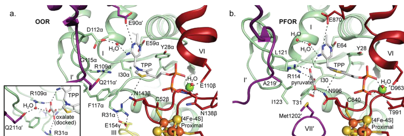
Figure 4. Active sites of OOR and Da PFOR. (a) The active site of OOR is shown with TPP in the middle and the substrate-binding pocket directly to the left, bounded by Arg109α, Gln211α', Phe117α, Arg31α, and Asn143β. Some solvent molecules have been omitted for the sake of clarity. Domains are labeled and colored as in Figure 2. Cofactors and select residue side chains are labeled and shown as sticks. Coordination to Mg 2+ (green sphere) and other important short interatomic distances (less than ~4 Å) are shown with dashed lines. The inset shows a docking model for oxalate binding based on pyruvate binding in PFOR. Short interatomic distances to the docked oxalate are shown with dashed lines. A water molecule omitted in the main figure is shown here interacting with Arg109α, Gln211α', and the docked oxalate molecule. (b) The active site of PFOR (PDB entry 2C42) has TPP, the proximal [4Fe-4S] cluster, and bound pyruvate shown as sticks. Domains are labeled and colored as follows: I, green; VI, red; I' and VII', purple. Coordination to Mg 2+ (green sphere) and other important short interatomic distances (less than ~4 Å) are indicated with dashed lines.
